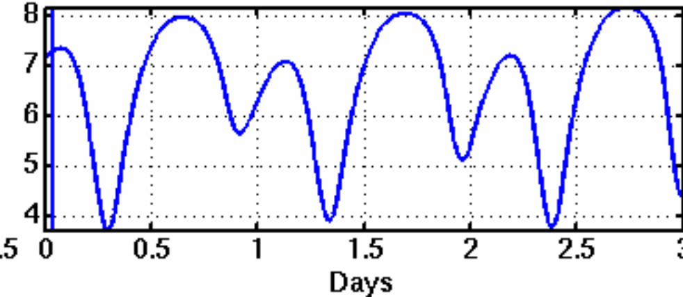
Discharge at Beaver Army (1000 m³/s)
