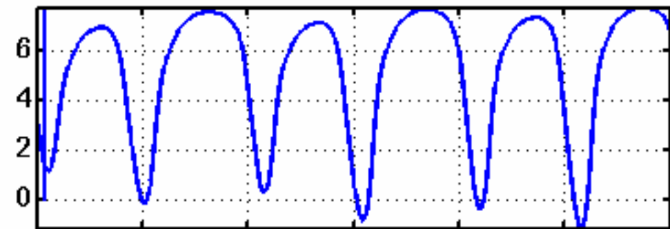
Discharge at Beaver Army (1000 m 3 /s)
