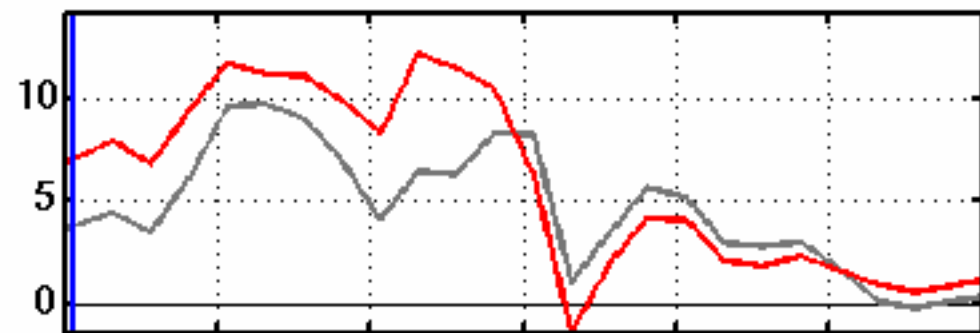
N-S Winds at SATURN02, 46029 (m/s)
