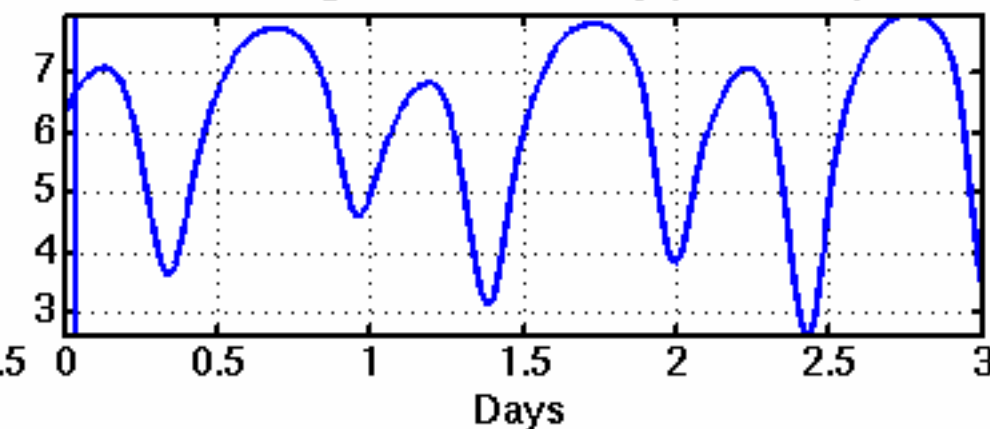
Discharge at Beaver Army (1000 m 3 /s)
