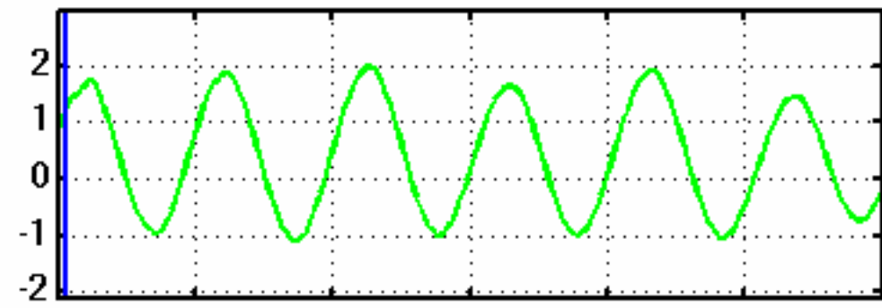
Discharge at Beaver Army (1000 m 3 /s)
