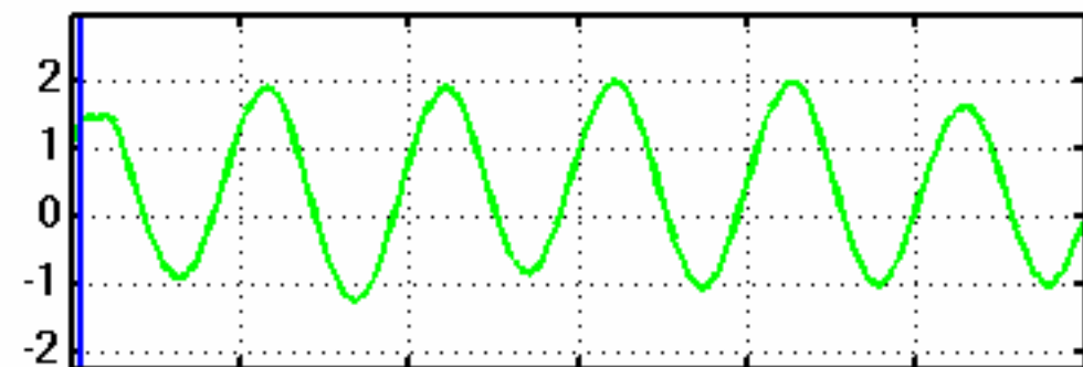
Tongue Point Elevations (m)
