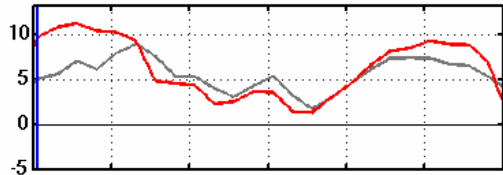
Tongue Point Elevations (m)
