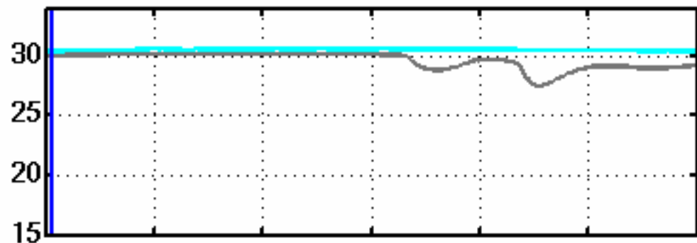
N-S Winds at SATURN02, 46029 (m/s)
