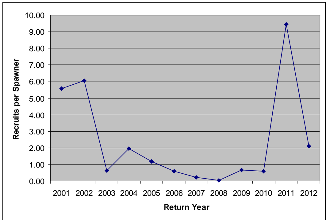
Figure 4. Trend in recruits per spawner for Coos Basin wild Coho Salmon, 2001-2012.
